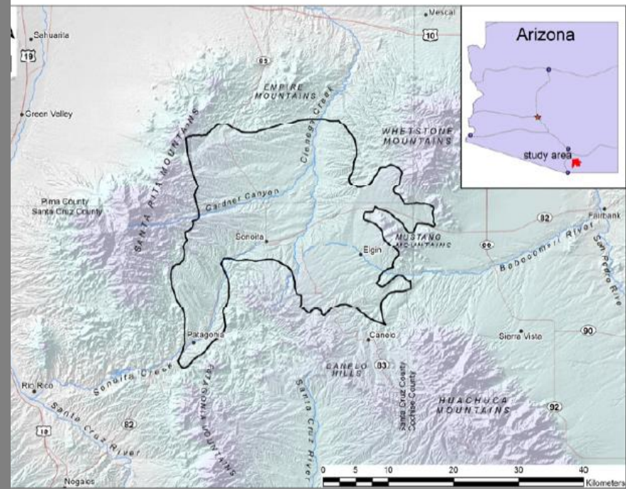
. Map of the Sonoita Plain, highlighting the mountains surrounding the study area.
